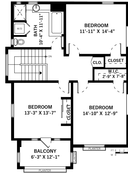
Upper Floor: 960 Sq.Ft. Ceiling Height: 8'-6"
